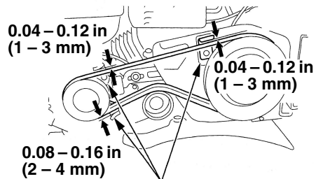
BELT STOPPER
