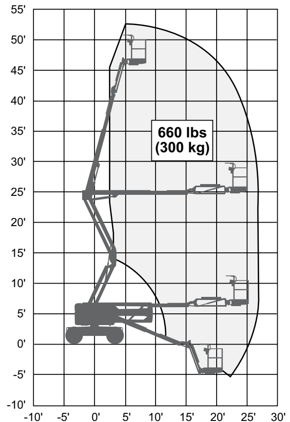
SJ46 AJ+ WORKING ENVELOPE
